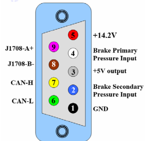
Figure 2 - DB9 female connector
