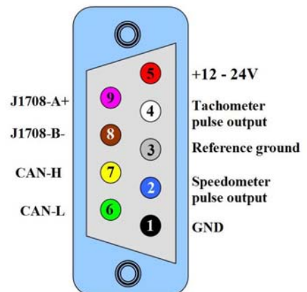
Figure 2 - DB9 female connector
